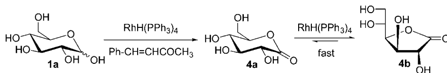
Scheme 2. Oxidation and isomerization of D-glucose to the \delta - and \gamma -lactones
