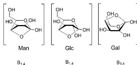
Figure 3. Structures of the proposed bicyclic intermediates in the \gamma \rightarrow \delta isomerization reactions of mannono-, glucono-, and galactonolactone
