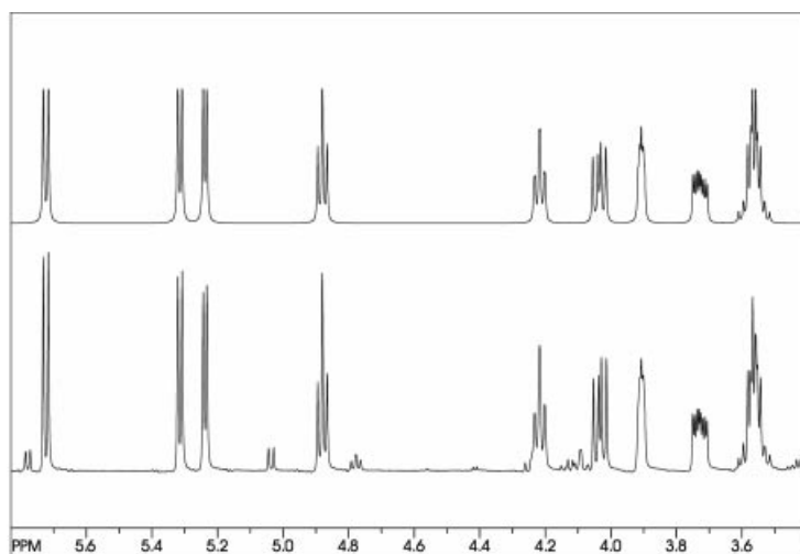
Figure 1. Simulated and experimental {}^1\text{H} NMR spectra of 6a , displaying the range between \delta = 3.4 and 5.8 ppm, using TMS as an internal standard
