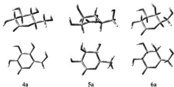
Figure 2. “Side” and “top” views of the minimum energy conformations of \delta -gluco ( 4a ), \delta -manno ( 5a ), and \delta -galactono ( 6a ) lactones determined by DFT [ mPW1PW91 /6–31(d,p)] calculations
