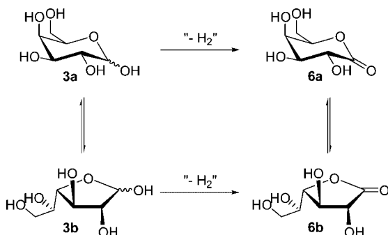
Scheme 1. Possible pathways for the oxidation of galactose ( 3 ) to the lactones 6a,b
